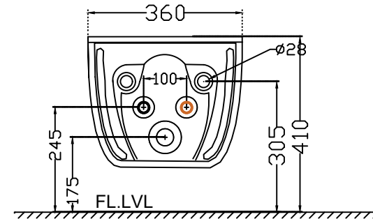
BACK VIEW A
