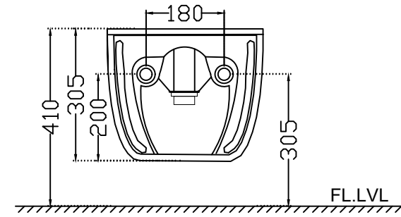
BACK VIEW
